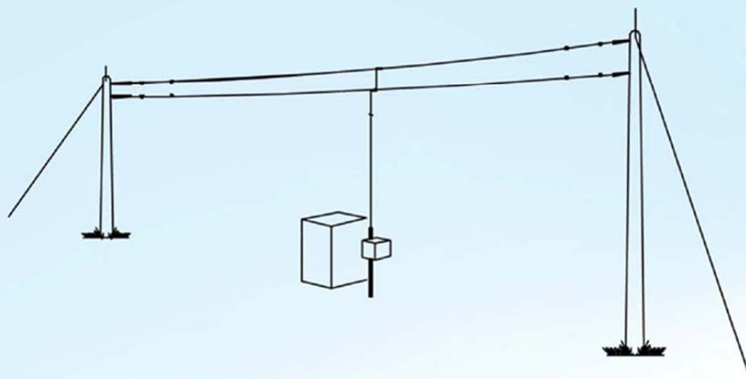
90' Symmetrical T Antenna Setup
